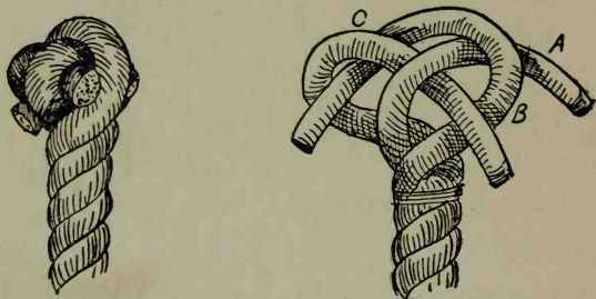
FIG. 110.—Single crown. FIG. 111.—Single crown (making).
